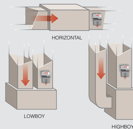
Duct Direct-Mount
