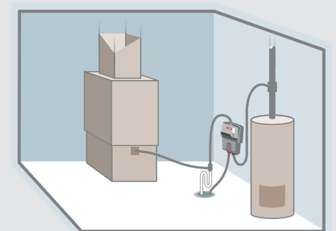
Down-Flow Remote-Mount
