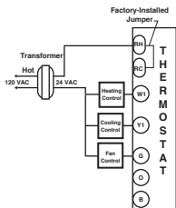
HEAT/COOL 4-WIRE SINGLE TRANSFORMER
