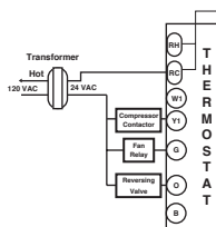
HEAT PUMP WITH COOL ACTIVE REVERSING VALVE
