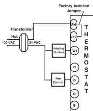
HEAT ONLY 3-WIRE SINGLE TRANSFORMER
