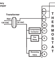
HEAT PUMP WITH HEAT ACTIVE REVERSING VALVE
