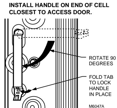
Fig. 17. Install handle on end of cell closest to access door.
