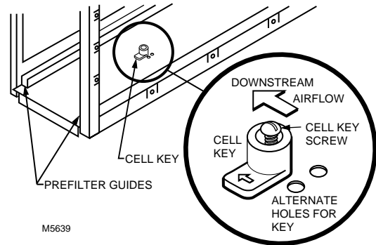
Fig. 16. Position of cell key determines orientation of cell (arrow on key must point downstream).
