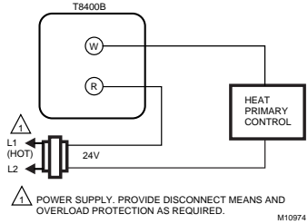
Fig. 5. T8400B heat-only wiring diagram in a single transformer system with gas heat.
