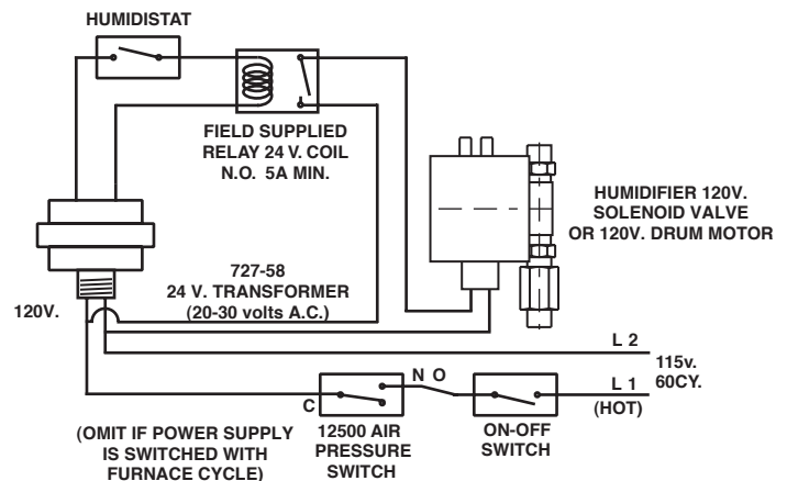
DIAGRAM 2 WIRING 120V. BYPASS HUMIDIFIER
