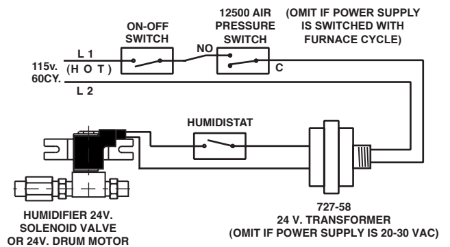
DIAGRAM 2 WIRING 120V. BYPASS HUMIDIFIER
