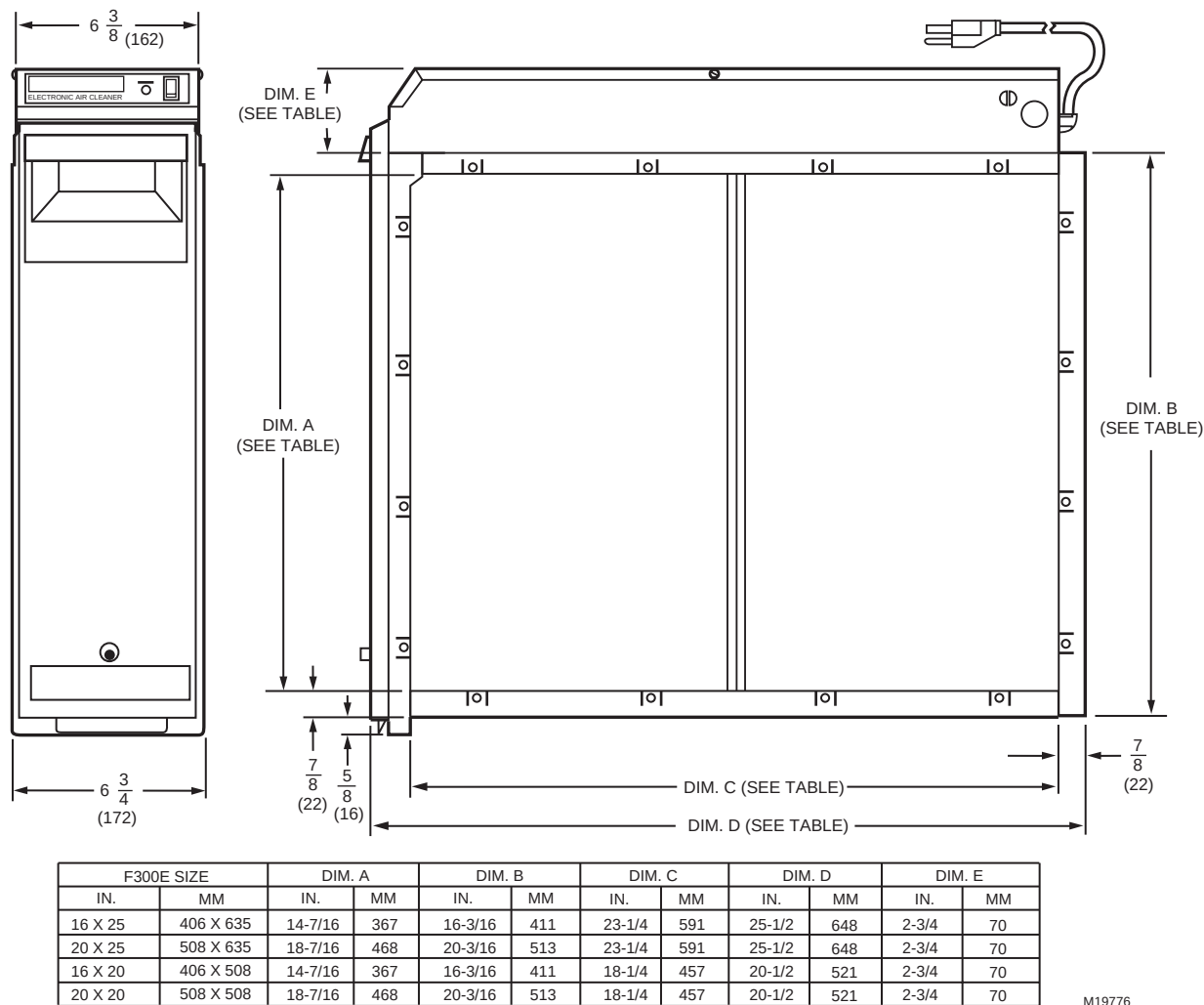
Fig. 1. Electronic Air Cleaner installation dimensions in in. (mm).
