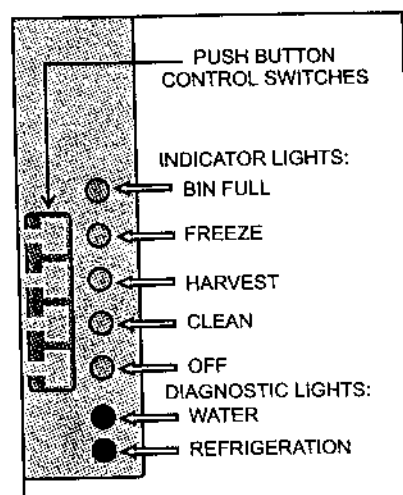
Controller Lights
